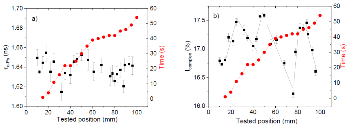
Fig. 1. Dependence of o -Ps lifetime (a) and complex intensity (b) on the tested position of the cured BADGE sample (the tested position is the point where the frontal wave was localized in time from start of reaction). Adapted from [1].
