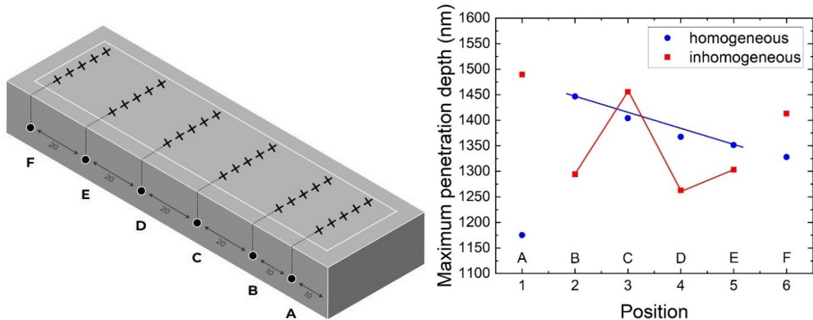
Fig. 2. Dependence of the maximum penetration depth in nanoindentation measurements with the UNHT on the tested position of the cured BADGE homogeneous and inhomogeneous samples (the tested position: 1-A – 10 mm, 2-B – 20 mm, 3-C – 40 mm, 4-D – 60 mm, 5-E – 80 mm, and 6-F – 100 mm, is the point where the frontal wave was localized in time from start of reaction).
